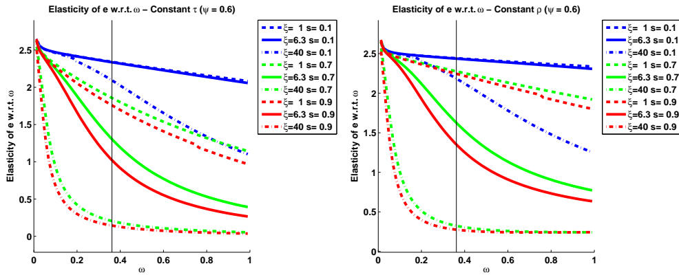
Figure 3: Elasticity of e with respect to \omega
