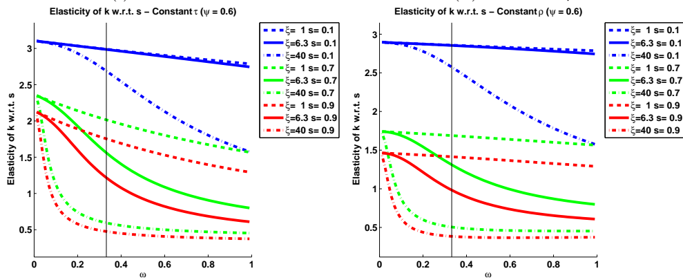
Figure 4: Elasticity of k with respect to s : No Annuity Markets
