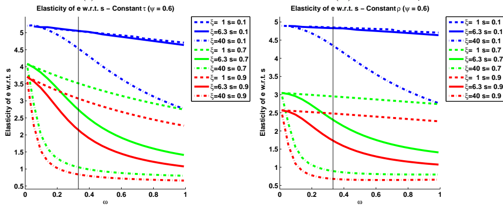
Figure 5: Elasticity of e with respect to s : No Annuity Markets
