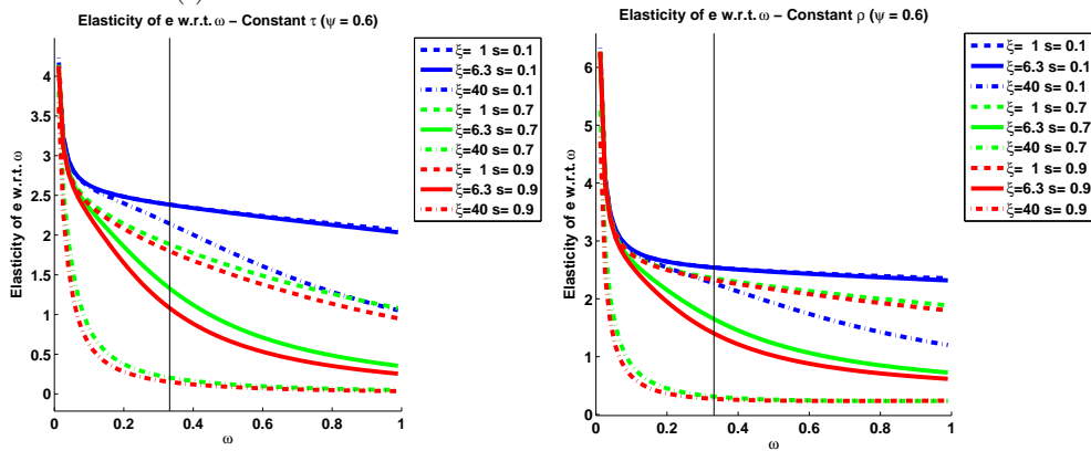
Figure 6: Elasticity of e with respect to \omega : No Annuity Markets
