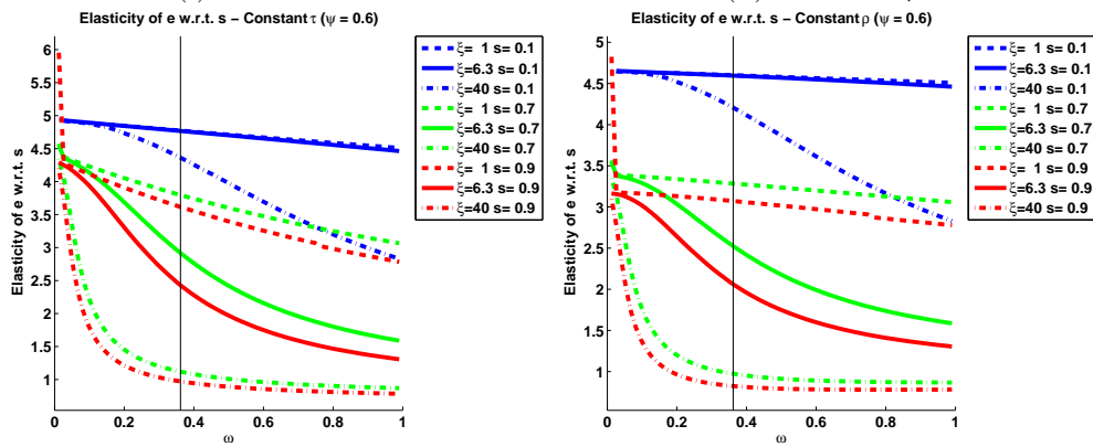
Figure 2: Elasticity of e with respect to s
