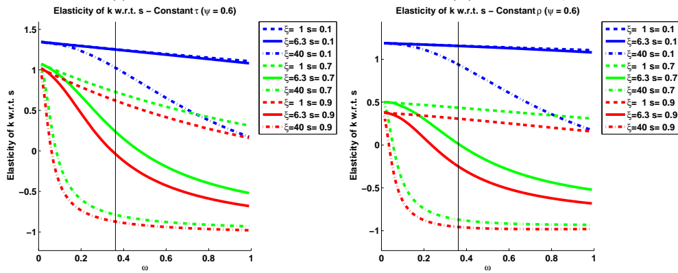
Figure 1: Elasticity of k with respect to s
